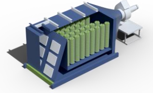
Filter Media
